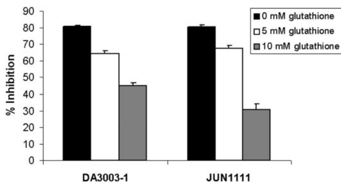
Fig. 7. Glutathione decreases the potency of DA3003-1 and JUN1111. In vitro inhibition of Cdc25B phosphatase by DA3003-1 (1.56 \mu M) and JUN1111 (3.13 \mu M) was tested in the presence of increasing concentrations of glutathione (0, 5, and 10 mM). Results are mean \pm S.E.M. ( n = 6 ). A negative correlation of -1 (effect of glutathione on percentage of inhibition of enzyme) was determined by Spearman's rank correlation.
