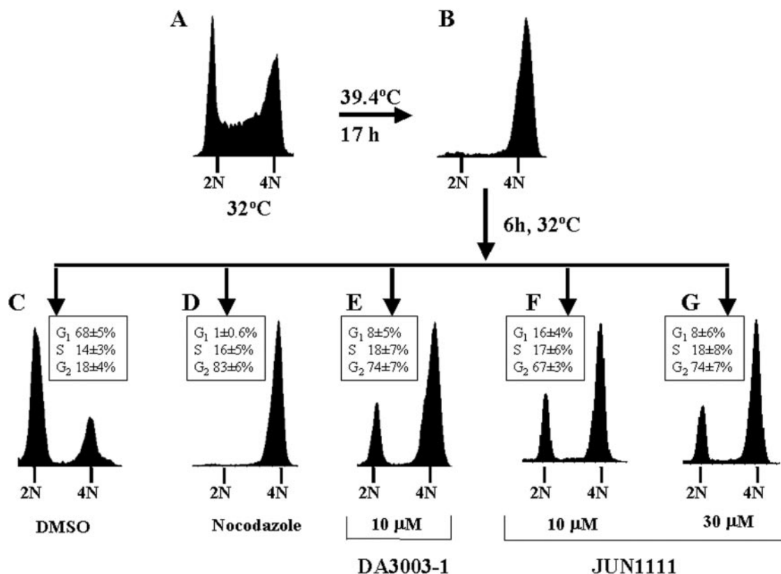
Fig. 2. G 2 /M arrest with DA3003-1 and JUN1111. tsFT210 cells were cultured at the permissive temperature of 32°C and then incubated for 17 h at the nonpermissive temperature (39.4°C). DMSO or drug was added to cells for an additional 6 h at 32°C. A, asynchronous control. B, G 2 /M-arrested cells after temperature shift for 17 h at 39.4°C. C, DMSO-treated cells. D, cells treated with 1 \mu M nocodazole (positive control). E, cells treated with 10 \mu M DA3003-1. F and G, cells treated with 10 or 30 \mu M JUN1111. Data are representative of three independent experiments.
