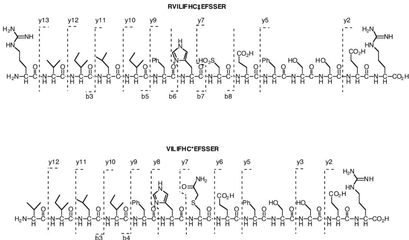
Fig. 9. Fragmentation patterns for peptides generated from tryptic digests of Cdc25B 2 incubated with DMSO vehicle or with a 30-fold molar excess of DA3003-1 for MALDI-TOF-MS spectra analysis. RVILIFHC 46 *EFSSER (* is Cys-sulfonic acid) treated with DA3003-1. VILIFHC 46 *EFSSER (* is carbamidomethylated) containing the iodoacetamide-blocked active site cysteine.
