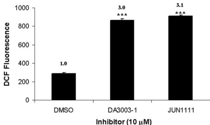
Fig. 8. DA3003-1 and JUN1111 produce ROS in cells. tsFT210 cells were preloaded with DCF dye (to measure ROS) and propidium iodide (to measure cell death) before treatment with DMSO, DA3003-1 (10 \mu M), or JUN1111 (10 \mu M) for 10 min. Resulting DCF and PI fluorescence was measured by flow cytometry. Results are mean \pm S.E.M. ( n = 3 ). Statistical significance was assessed by one-way analysis of variance. ***, p < 0.001 compared with DMSO control.
