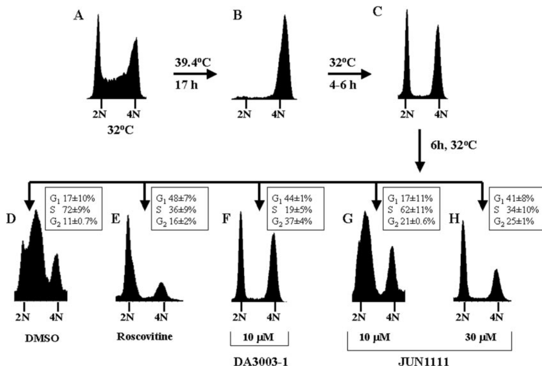
Fig. 1. G_1 phase arrest with DA3003-1 and JUN1111. tsFT210 cells were cultured at the permissive temperature of 32°C and then incubated at the nonpermissive temperature (39.4°C) for 17 h to synchronize cells at G_2/M . Cells were then released for 4 to 6 h at 32°C to arrest cells at the G_1 checkpoint. DMSO or inhibitor was added for an additional 6 h at 32°C. A, asynchronous control. B, G_2/M -arrested cells after temperature shift for 17 h at 39.4°C. C, G_1 -arrested cells after temperature shift back to 32°C. D, DMSO-treated cells. E, cells treated with 50 \mu\text{M} roscovitine (positive control). F, cells treated with 10 \mu\text{M} DA3003-1. G and H, cells treated with 10 or 30 \mu\text{M} JUN1111. Data are representative of three independent experiments.
