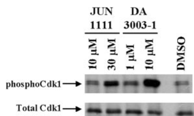
Fig. 3. Cdk1 is hyperphosphorylated in the presence of DA3003-1 and JUN1111. G_2/M -arrested tsFT210 cells were released for 1 h in the presence of 10 and 30 \mu M JUN1111 or 1 and 10 \mu M DA3003-1 or DMSO vehicle followed by immunoprecipitation with anti-Cdk1 mouse monoclonal antibody. Western blots were probed with phospho-Cdk1 (Tyr15) antibody. Blots were stripped and reprobed with total Cdk1 antibody as a loading control.
