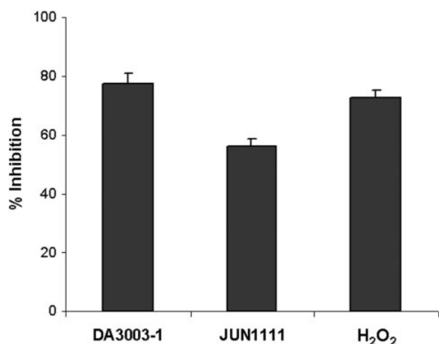
Fig. 4. DA3003-1 and JUN1111 directly inhibit transfected Cdc25B in HeLa cells. Transfected cells were treated with DA3003-1 (10 \mu M), JUN1111 (10 \mu M), or H 2 O 2 (1 mM) followed by immunoprecipitation of myc-Cdc25B. The remaining enzyme activity was tested in vitro using OMFP as a substrate. Percentage of inhibition was calculated by comparing to DMSO-treated myc-Cdc25B transfected cells (positive control) and DMSO-treated myc-vector transfected cells (negative control). Results are mean \pm S.E.M. ( n = 4 ).
