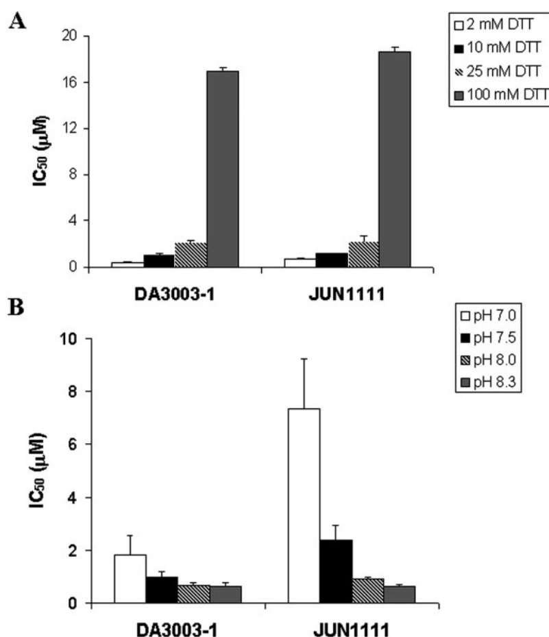
Fig. 6. Effect of DTT concentration and pH on phosphatase inhibition. A, Cdc25B phosphatase inhibition by DA3003-1 and JUN111 was tested using our in vitro enzyme assay as described under Materials and Methods at DTT concentrations of 2, 10, 25, and 100 mM. Results are mean \pm S.E.M. ( n \geq 3 ). B, Cdc25B phosphatase inhibition by DA3003-1 and JUN111 was tested using our in vitro enzyme assay as described under Materials and Methods under various pH conditions (pH 7–8.3). Results are mean \pm S.E.M. ( n = 3 ). IC 50 values were calculated using GraphPad Prism software. A positive correlation of +1 (effect of DTT on IC 50 ) and a negative correlation of -1 (effect of pH on IC 50 ) were determined by Spearman's rank correlation.
