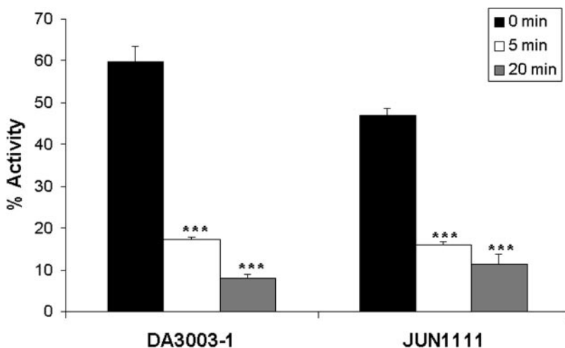
Fig. 4. DA3003-1 and JUN1111 directly inhibit transfected Cdc25B in HeLa cells. Transfected cells were treated with DA3003-1 (10 \mu M), JUN1111 (10 \mu M), or H 2 O 2 (1 mM) followed by immunoprecipitation of myc-Cdc25B. The remaining enzyme activity was tested in vitro using OMFP as a substrate. Percentage of inhibition was calculated by comparing to DMSO-treated myc-Cdc25B transfected cells (positive control) and DMSO-treated myc-vector transfected cells (negative control). Results are mean \pm S.E.M. ( n = 4 ).
